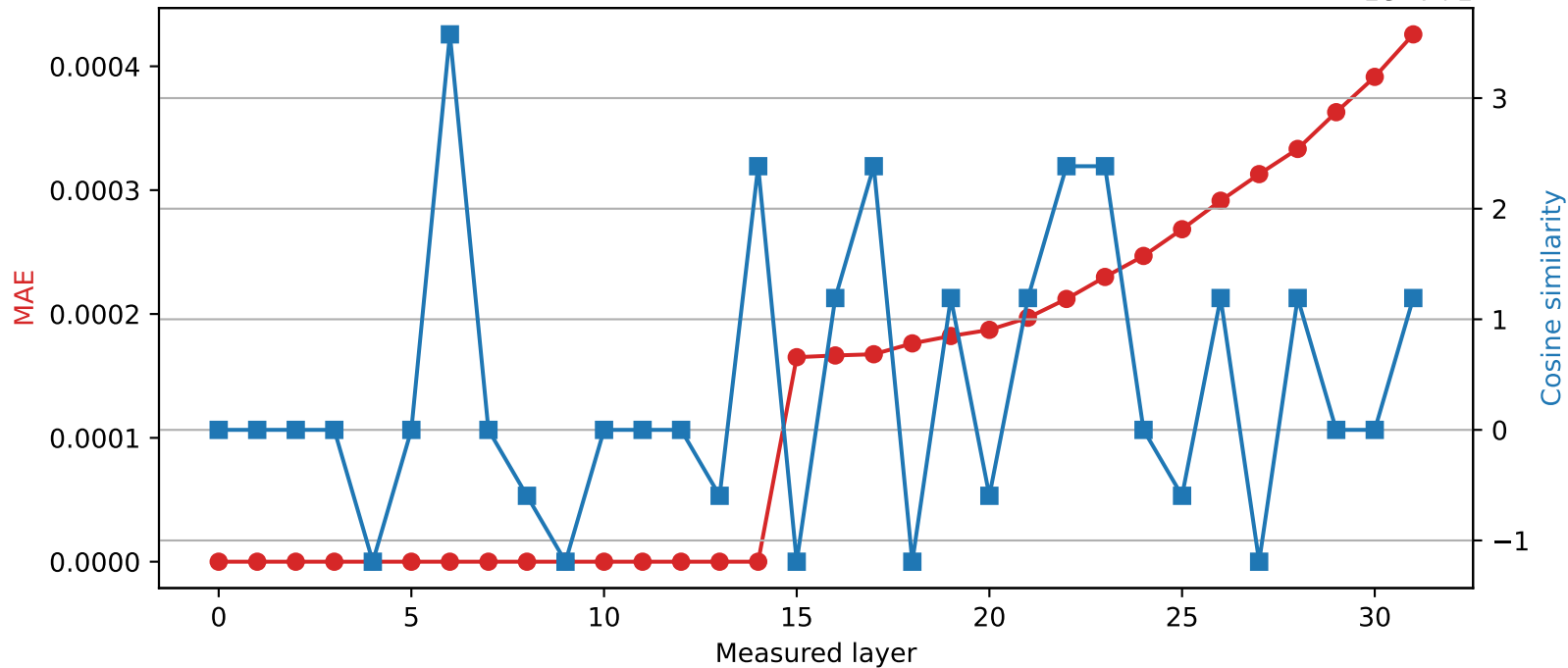
Phi-3-mini-4k-instruct | Quantized layer 14 | float64 → int16
