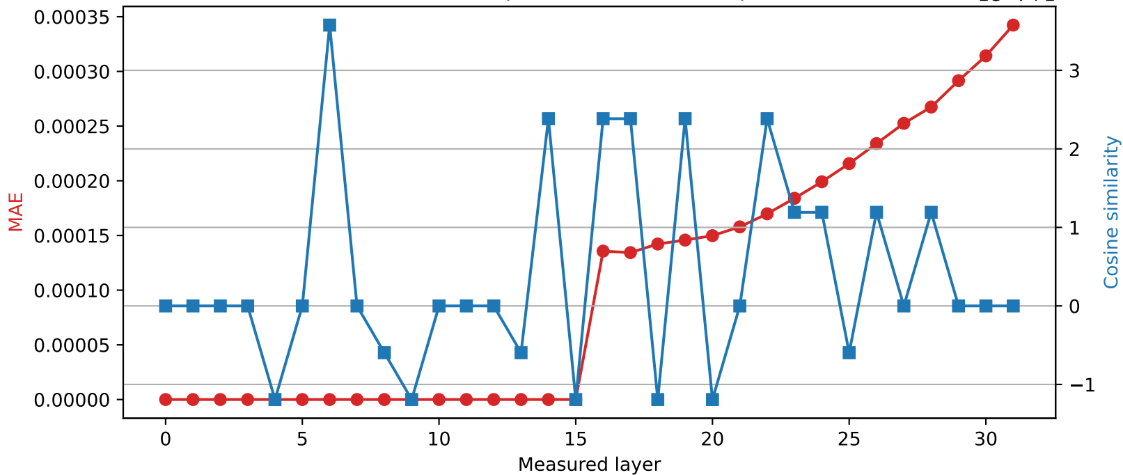
Phi-3-mini-4k-instruct | Quantized layer 15 | float64 \rightarrow int16
