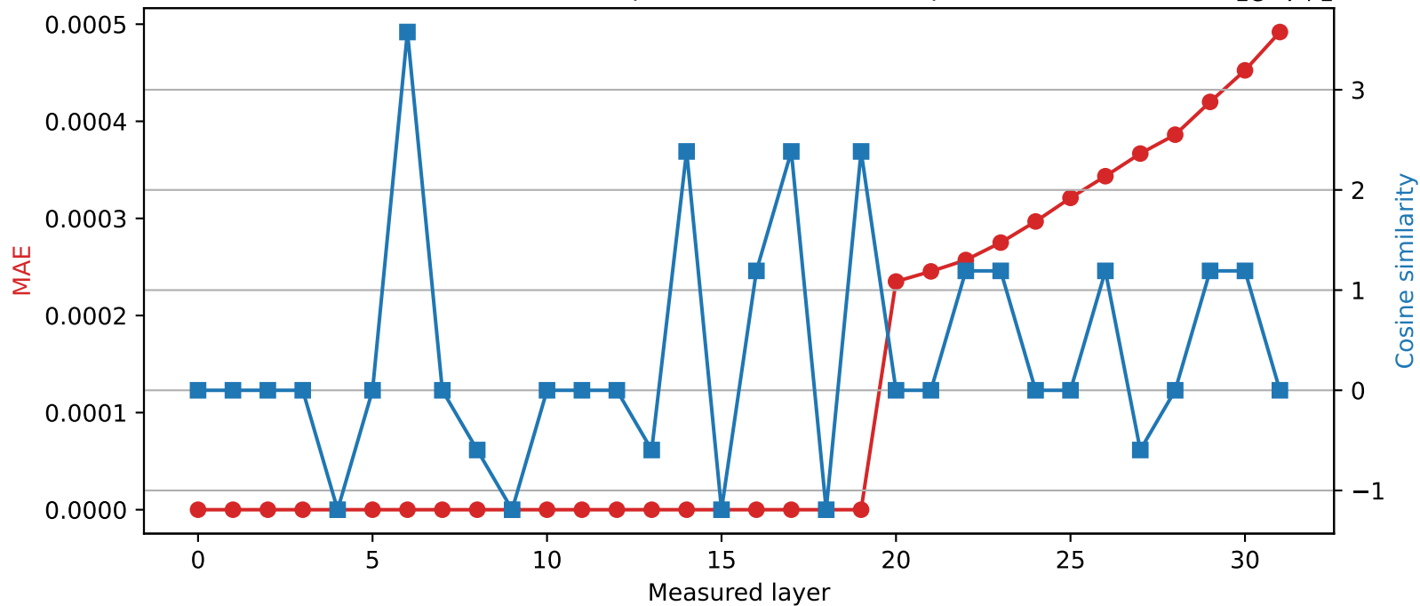
Phi-3-mini-4k-instruct | Quantized layer 19 | float64 → int16
