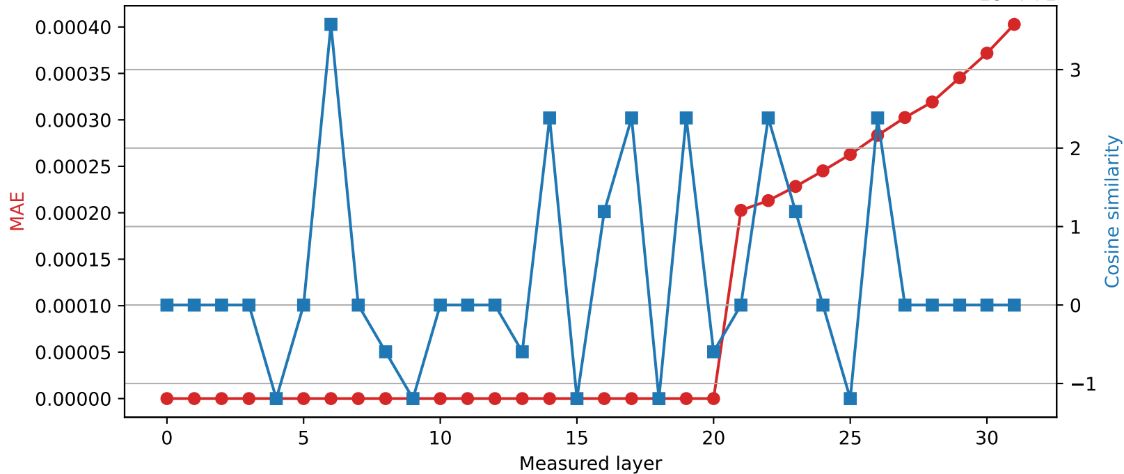
Phi-3-mini-4k-instruct | Quantized layer 20 | float64 → int16
