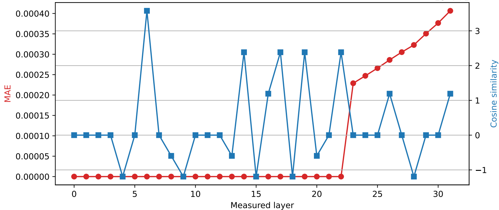
Phi-3-mini-4k-instruct | Quantized layer 22 | float64 → int16
