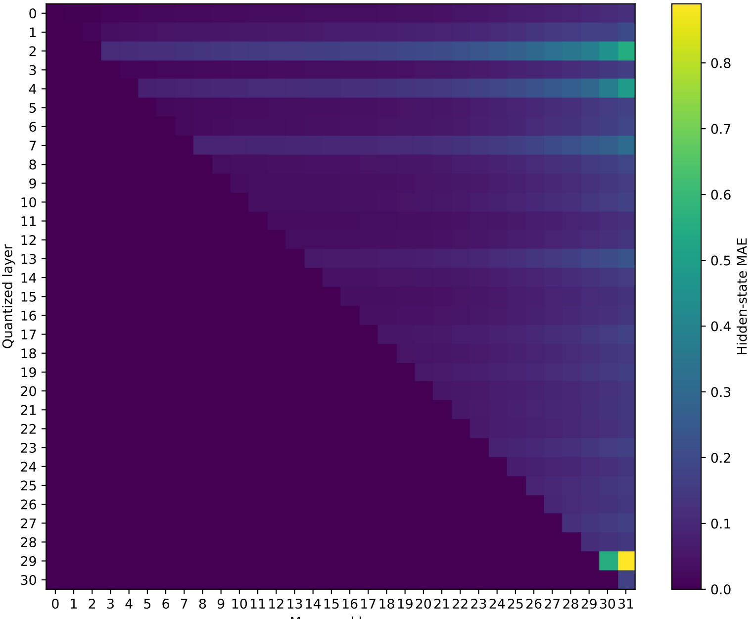
Model: Phi-3-mini-4k-instruct | float64 → int8
