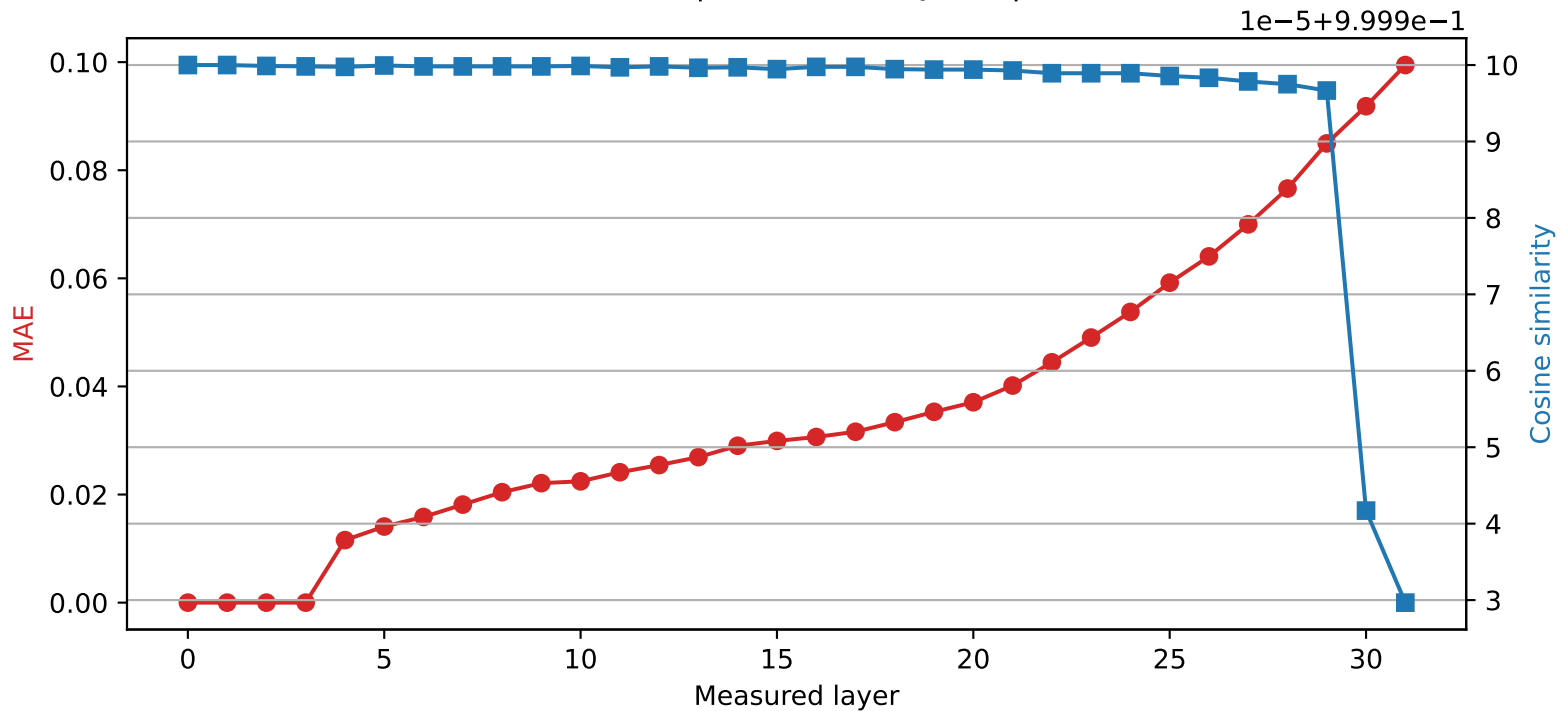
Phi-3-mini-4k-instruct | Quantized layer 3 | float64 → int8
