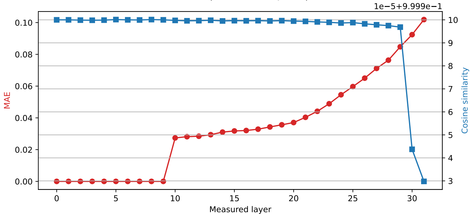
Phi-3-mini-4k-instruct | Quantized layer 9 | float64 → int8
