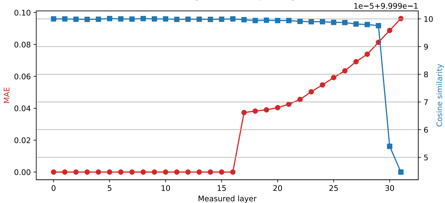
Phi-3-mini-4k-instruct | Quantized layer 16 | float64 → int8
