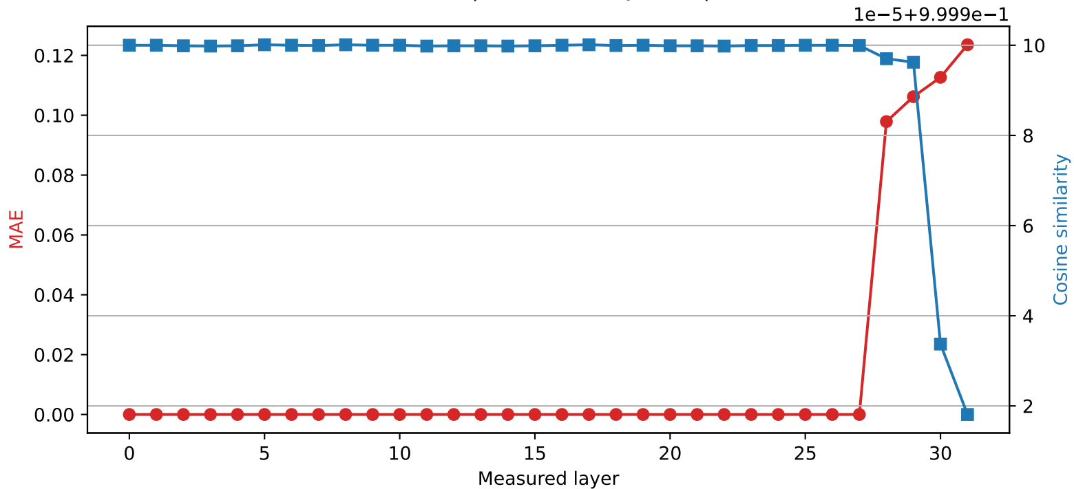
Phi-3-mini-4k-instruct | Quantized layer 27 | float64 \rightarrow int8
