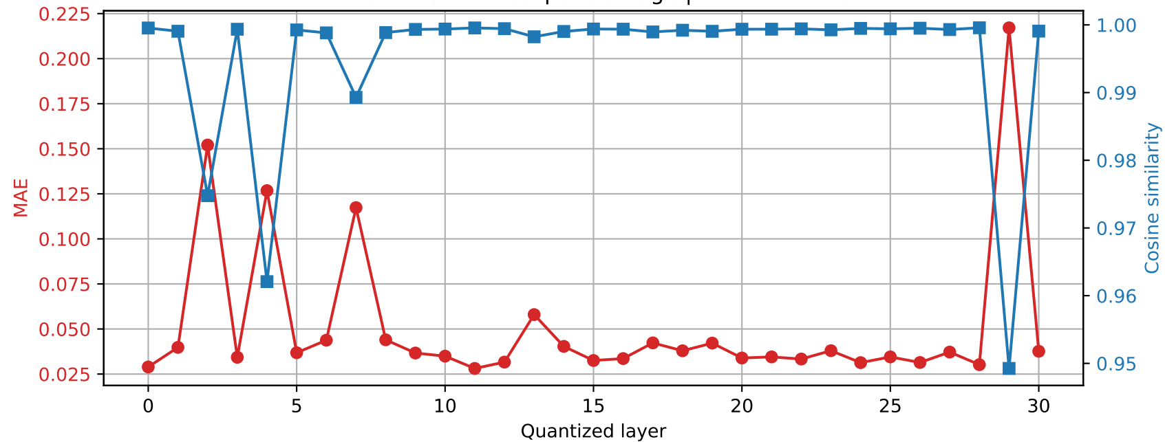
Phi-3-mini-4k-instruct | Prompt 1 Final RMSNorm output damage | float64 \rightarrow int8
