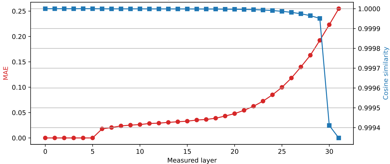
Phi-3-mini-4k-instruct | Quantized layer 5 | float64 \rightarrow int8
