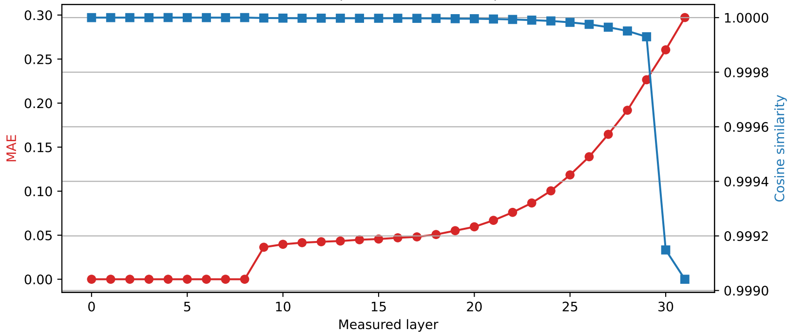
Phi-3-mini-4k-instruct | Quantized layer 8 | float64 \rightarrow int8
