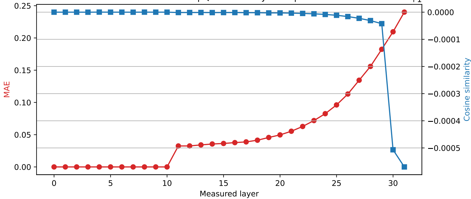
Phi-3-mini-4k-instruct | Quantized layer 10 | float64 \rightarrow int8
