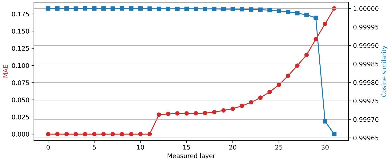
Phi-3-mini-4k-instruct | Quantized layer 11 | float64 \rightarrow int8
