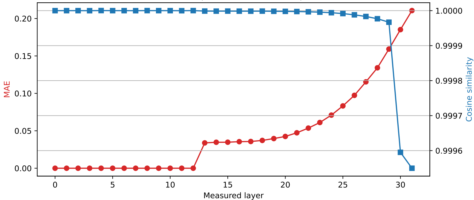
Phi-3-mini-4k-instruct | Quantized layer 12 | float64 \rightarrow int8
