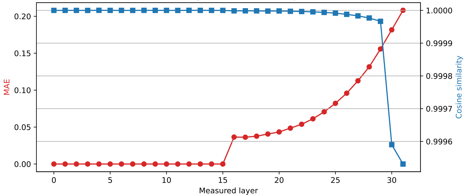
Phi-3-mini-4k-instruct | Quantized layer 15 | float64 \rightarrow int8
