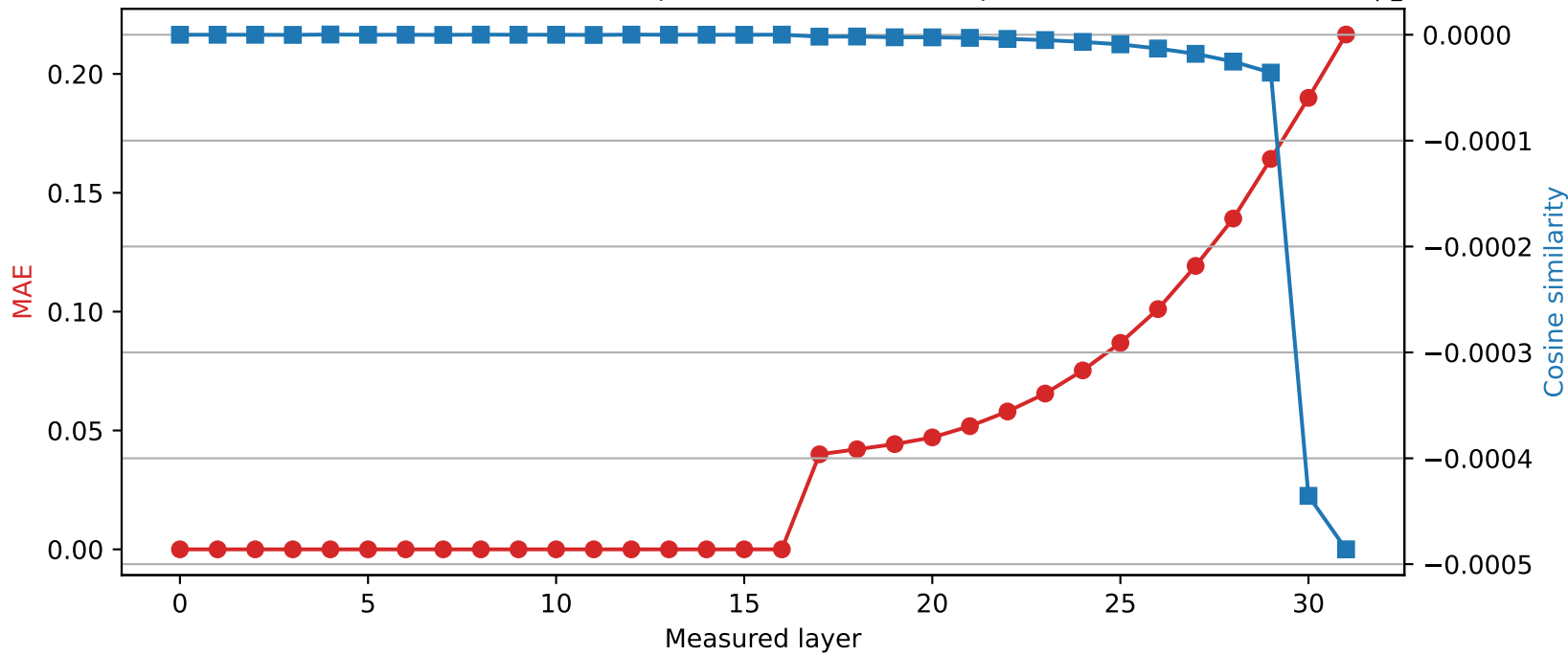
Phi-3-mini-4k-instruct | Quantized layer 16 | float64 \rightarrow int8
