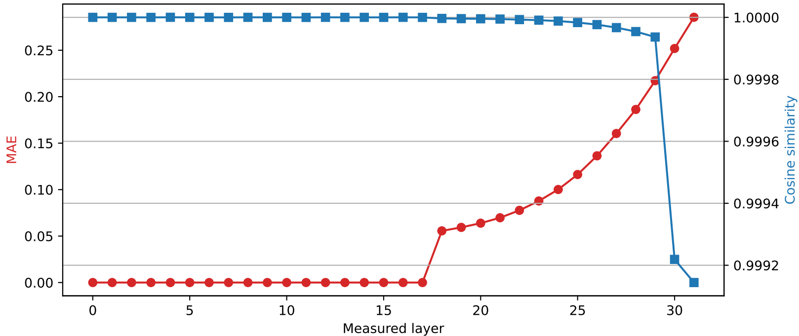
Phi-3-mini-4k-instruct | Quantized layer 17 | float64 \rightarrow int8
