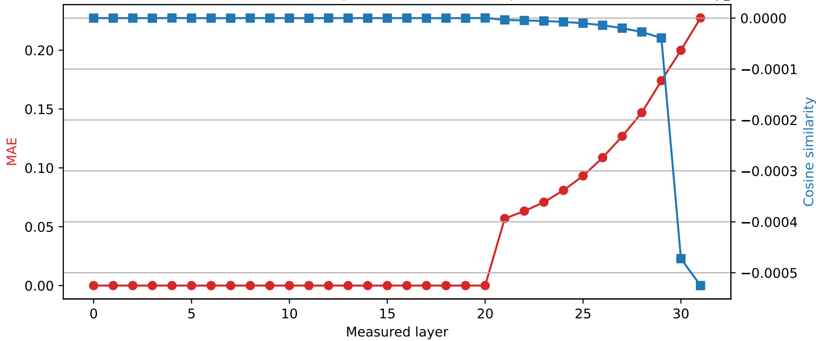
Phi-3-mini-4k-instruct | Quantized layer 20 | float64 \rightarrow int8
