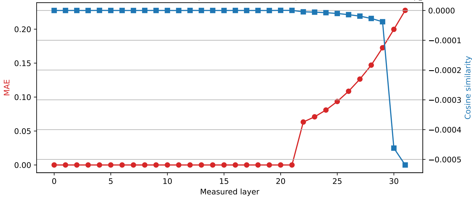
Phi-3-mini-4k-instruct | Quantized layer 21 | float64 \rightarrow int8
