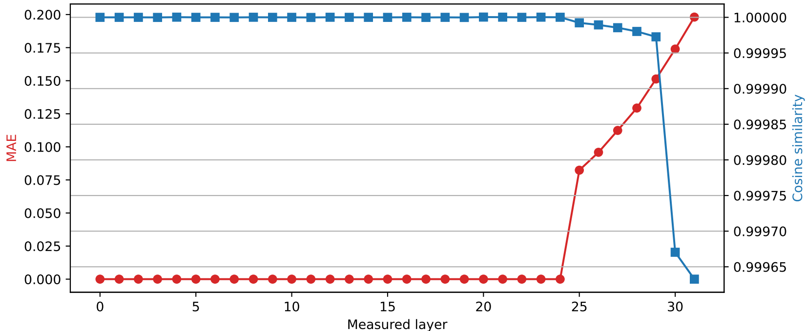
Phi-3-mini-4k-instruct | Quantized layer 24 | float64 \rightarrow int8
