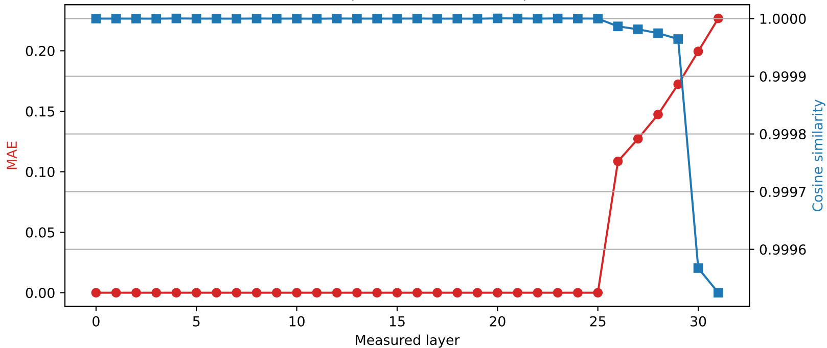
Phi-3-mini-4k-instruct | Quantized layer 25 | float64 \rightarrow int8
