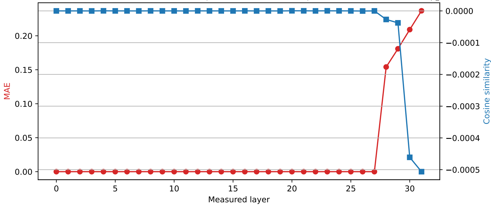
Phi-3-mini-4k-instruct | Quantized layer 27 | float64 \rightarrow int8
