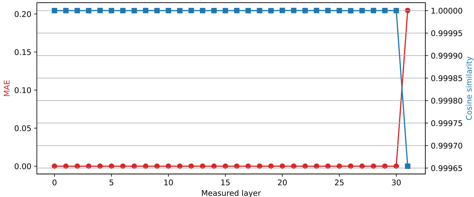
Phi-3-mini-4k-instruct | Quantized layer 30 | float64 \rightarrow int8
