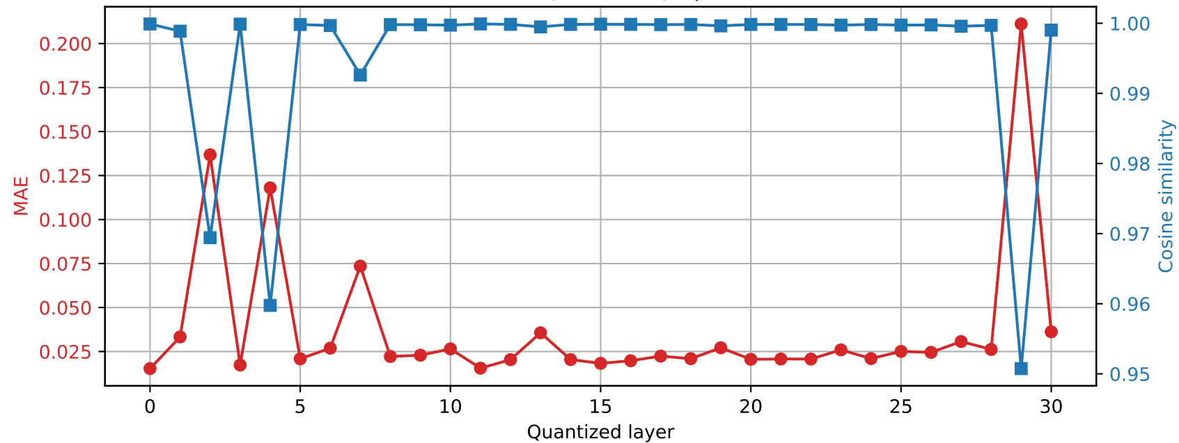
Phi-3-mini-4k-instruct | Prompt 2 Final RMSNorm output damage | float64 → int8
