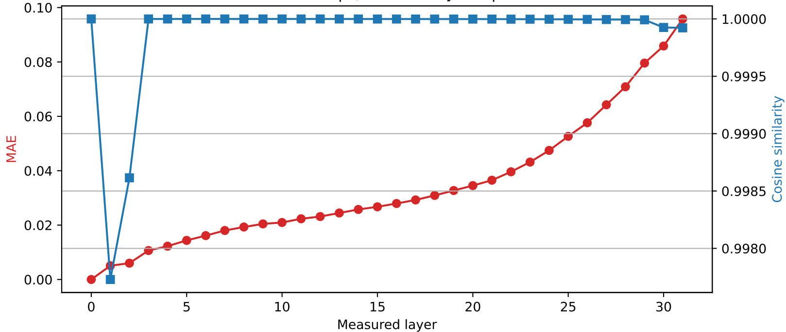
Phi-3-mini-4k-instruct | Quantized layer 0 | float64 \rightarrow int8
