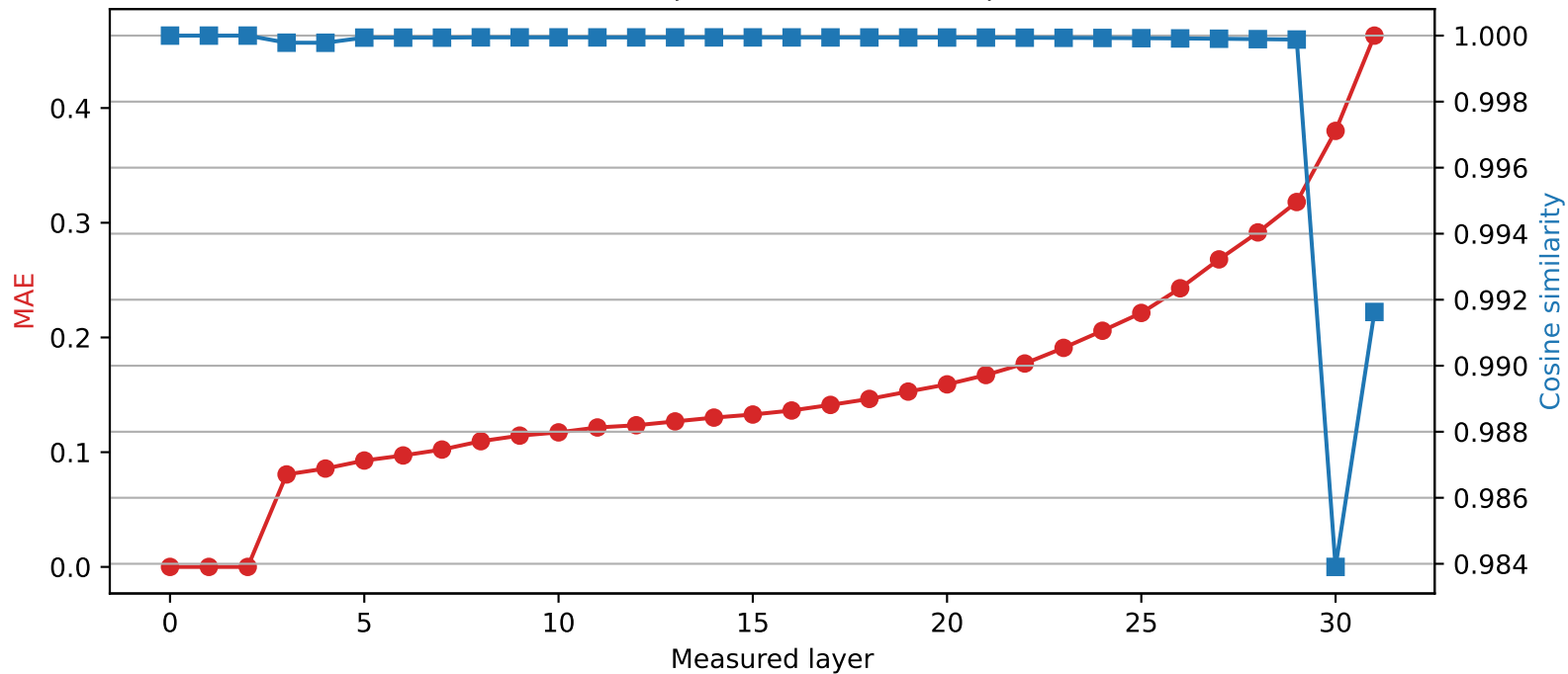
Phi-3-mini-4k-instruct | Quantized layer 2 | float64 \rightarrow int8
