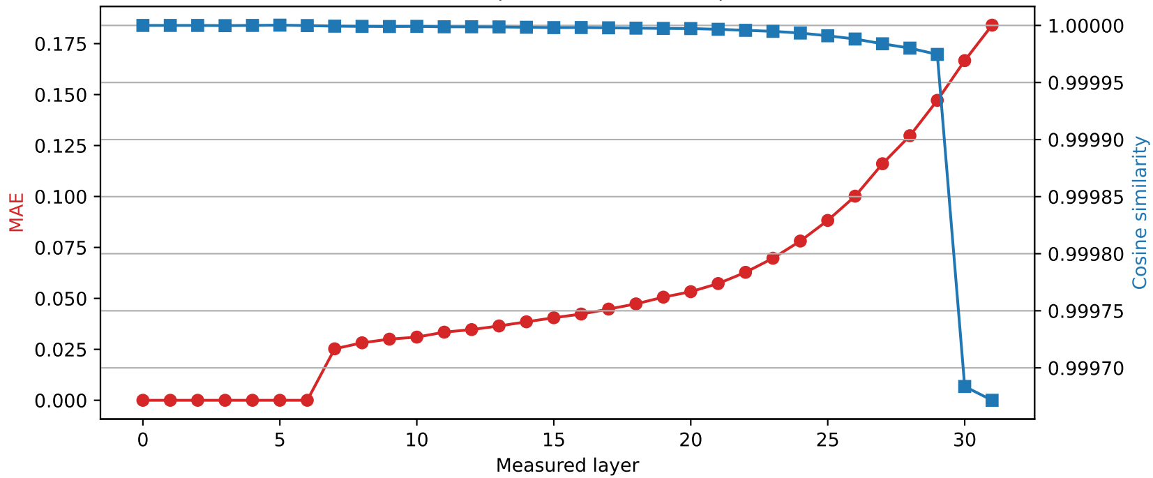
Phi-3-mini-4k-instruct | Quantized layer 6 | float64 → int8
