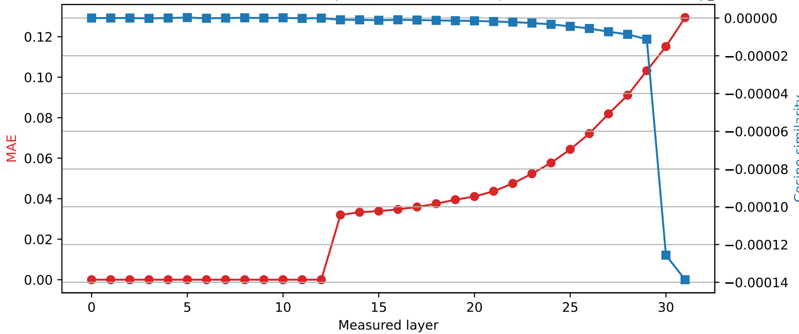
Phi-3-mini-4k-instruct | Quantized layer 12 | float64 → int8
