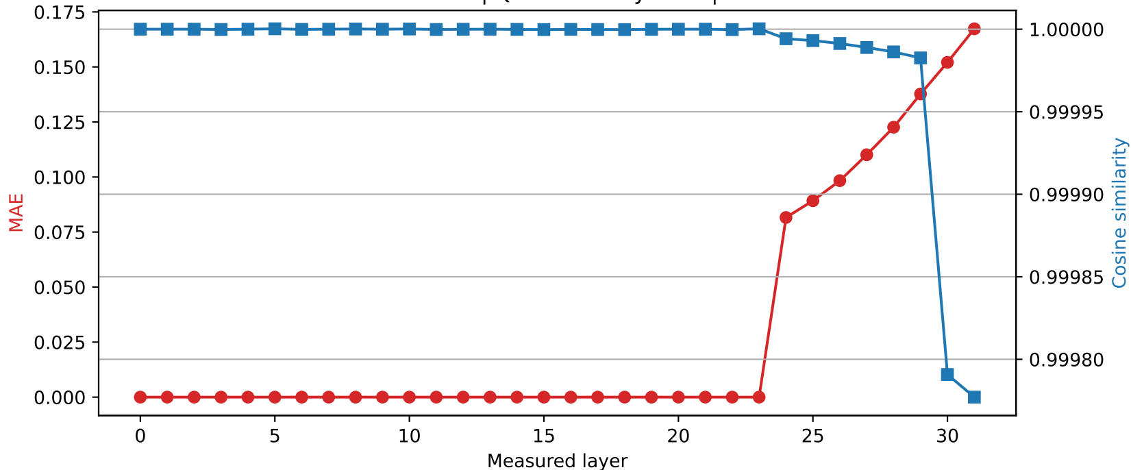
Phi-3-mini-4k-instruct | Quantized layer 23 | float64 \rightarrow int8
