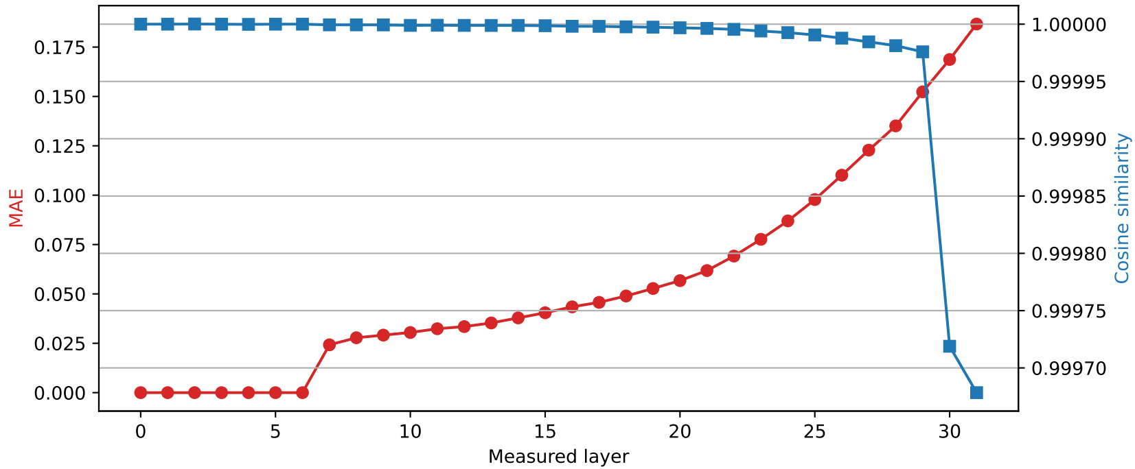
Phi-3-mini-4k-instruct | Quantized layer 6 | float64 \rightarrow int8
