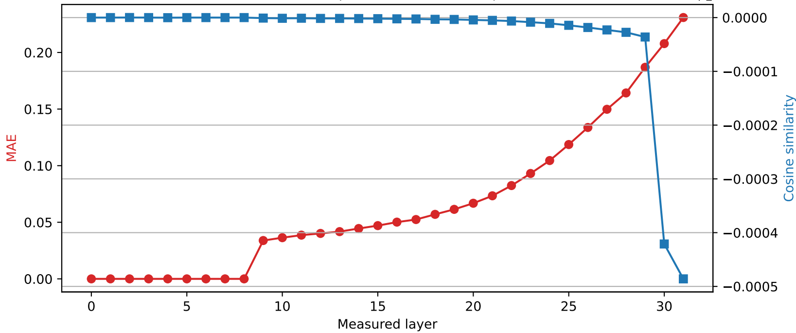
Phi-3-mini-4k-instruct | Quantized layer 8 | float64 \rightarrow int8
