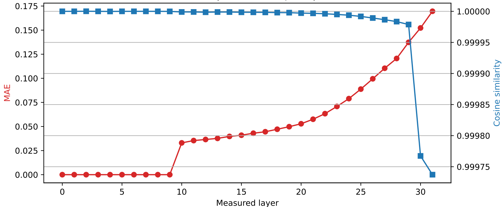
Phi-3-mini-4k-instruct | Quantized layer 9 | float64 \rightarrow int8
