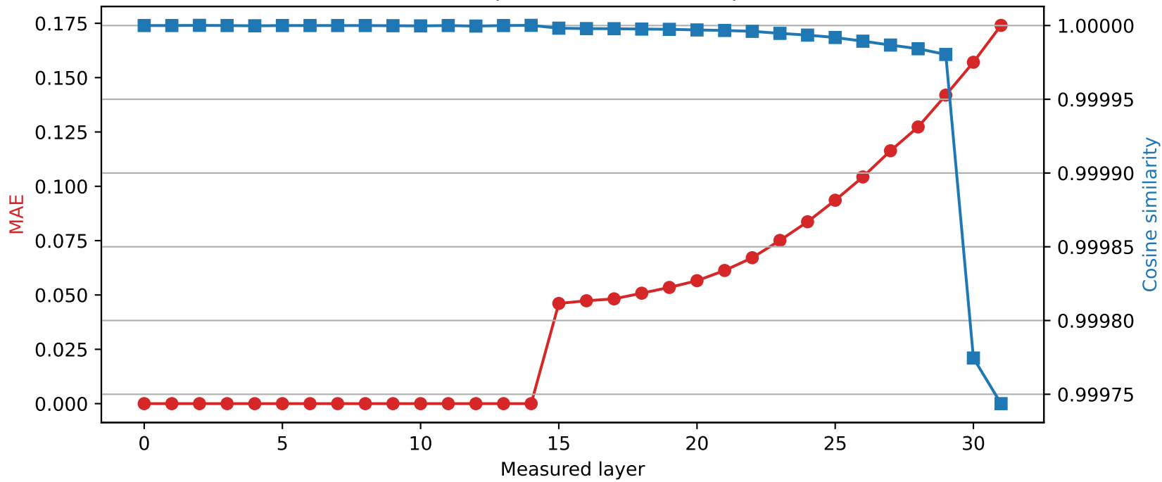
Phi-3-mini-4k-instruct | Quantized layer 14 | float64 \rightarrow int8
