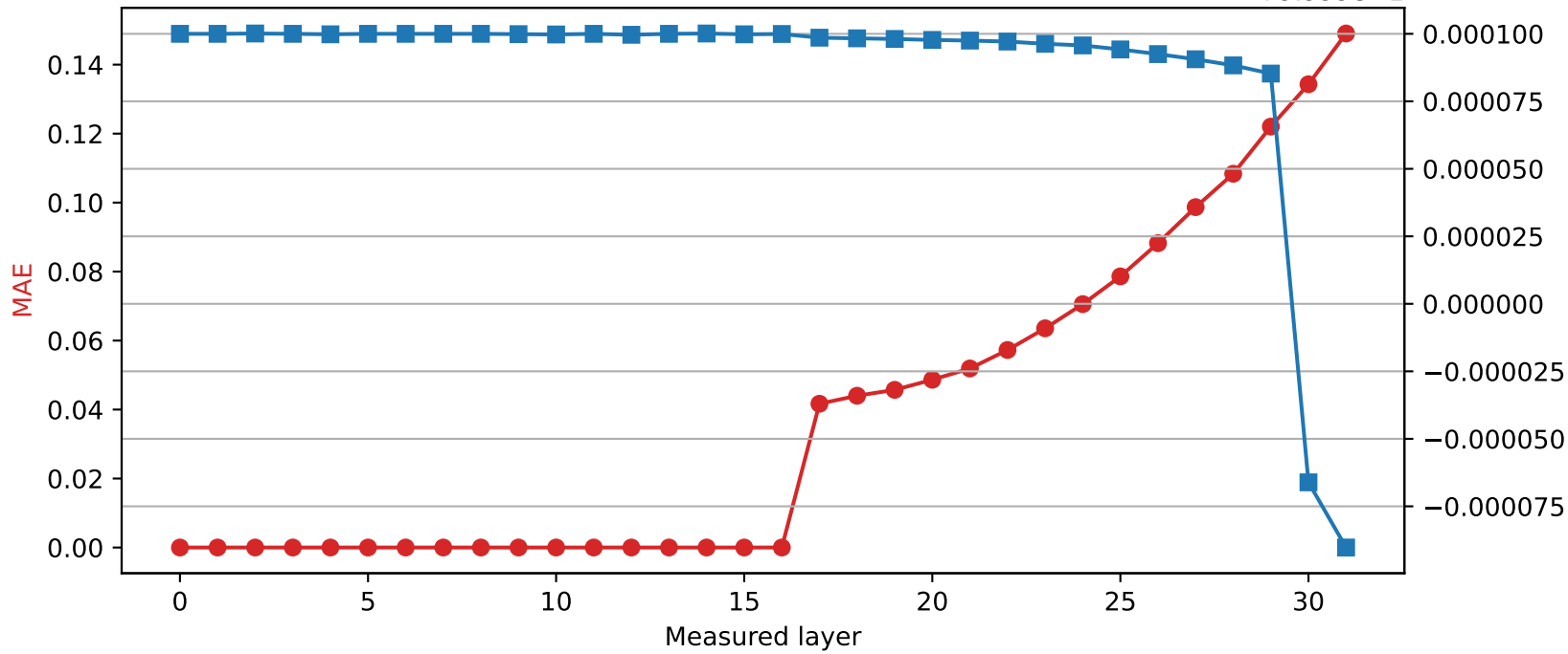
Phi-3-mini-4k-instruct | Quantized layer 16 | float64 → int8
