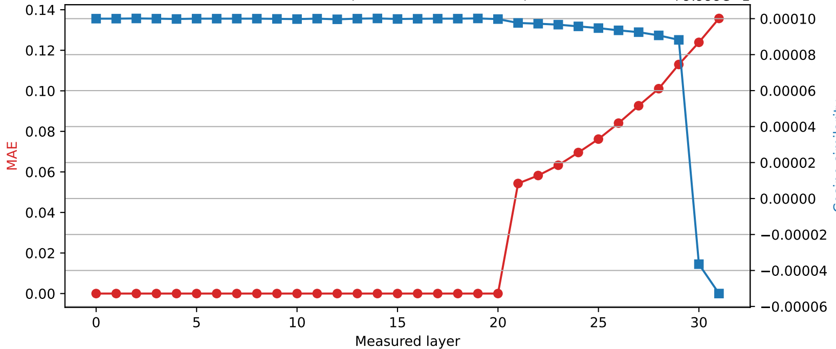
Phi-3-mini-4k-instruct | Quantized layer 20 | float64 → int8
