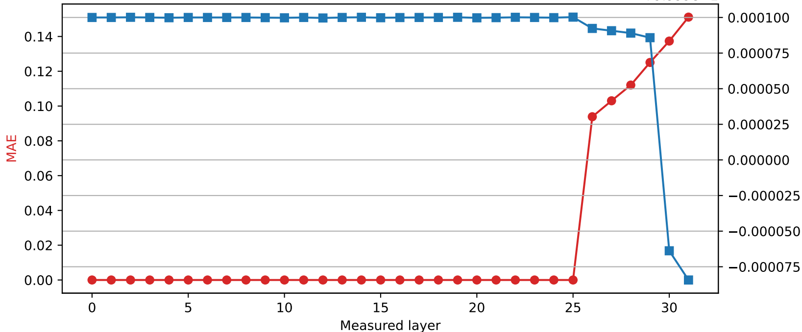
Phi-3-mini-4k-instruct | Quantized layer 25 | float64 \rightarrow int8
