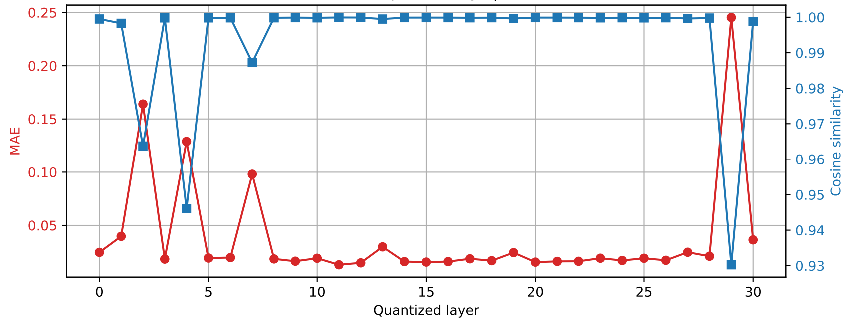
Phi-3-mini-4k-instruct | Prompt 4 Final RMSNorm output damage | float64 \rightarrow int8
