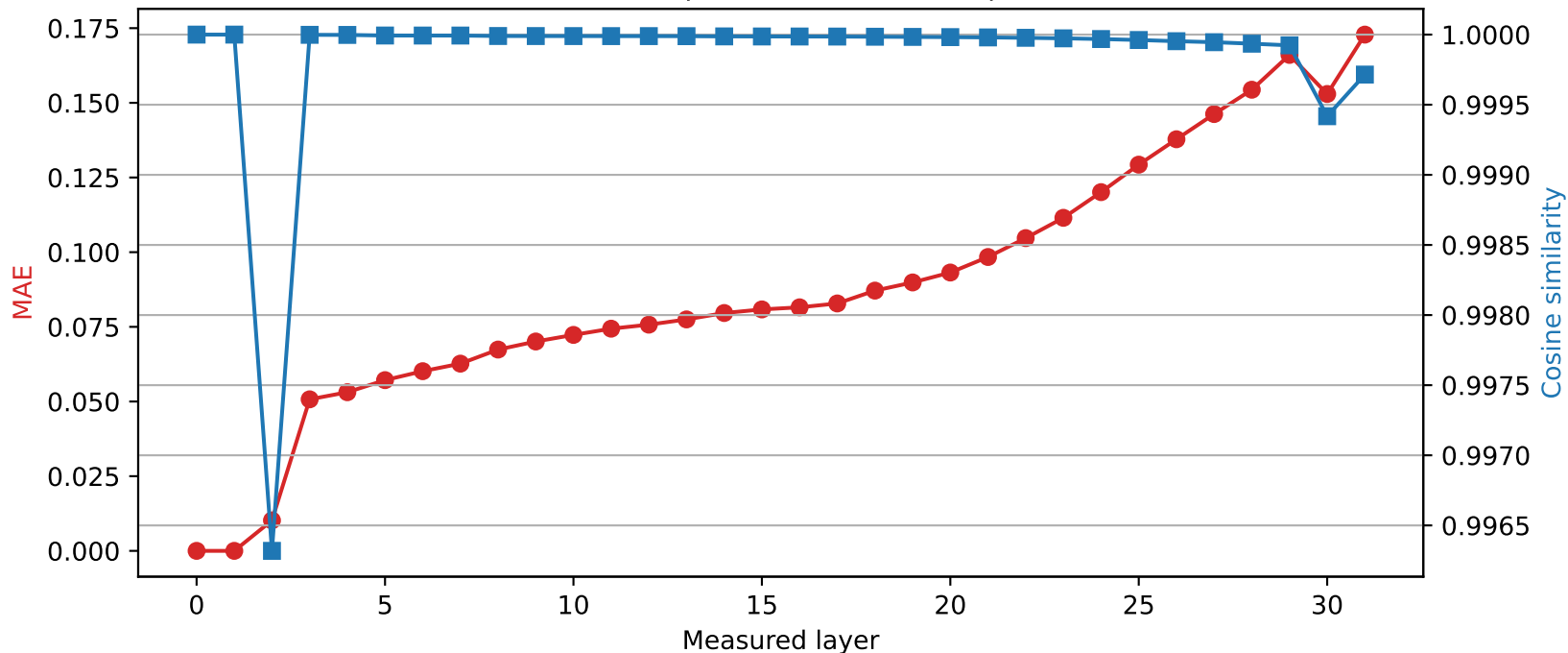
Phi-3-mini-4k-instruct | Quantized layer 1 | float64 \rightarrow int8
