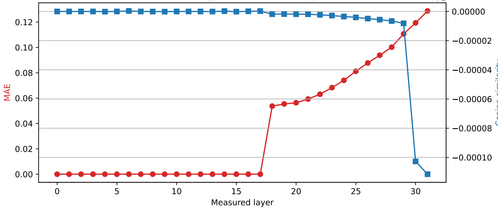
Phi-3-mini-4k-instruct | Quantized layer 17 | float64 \rightarrow int8
