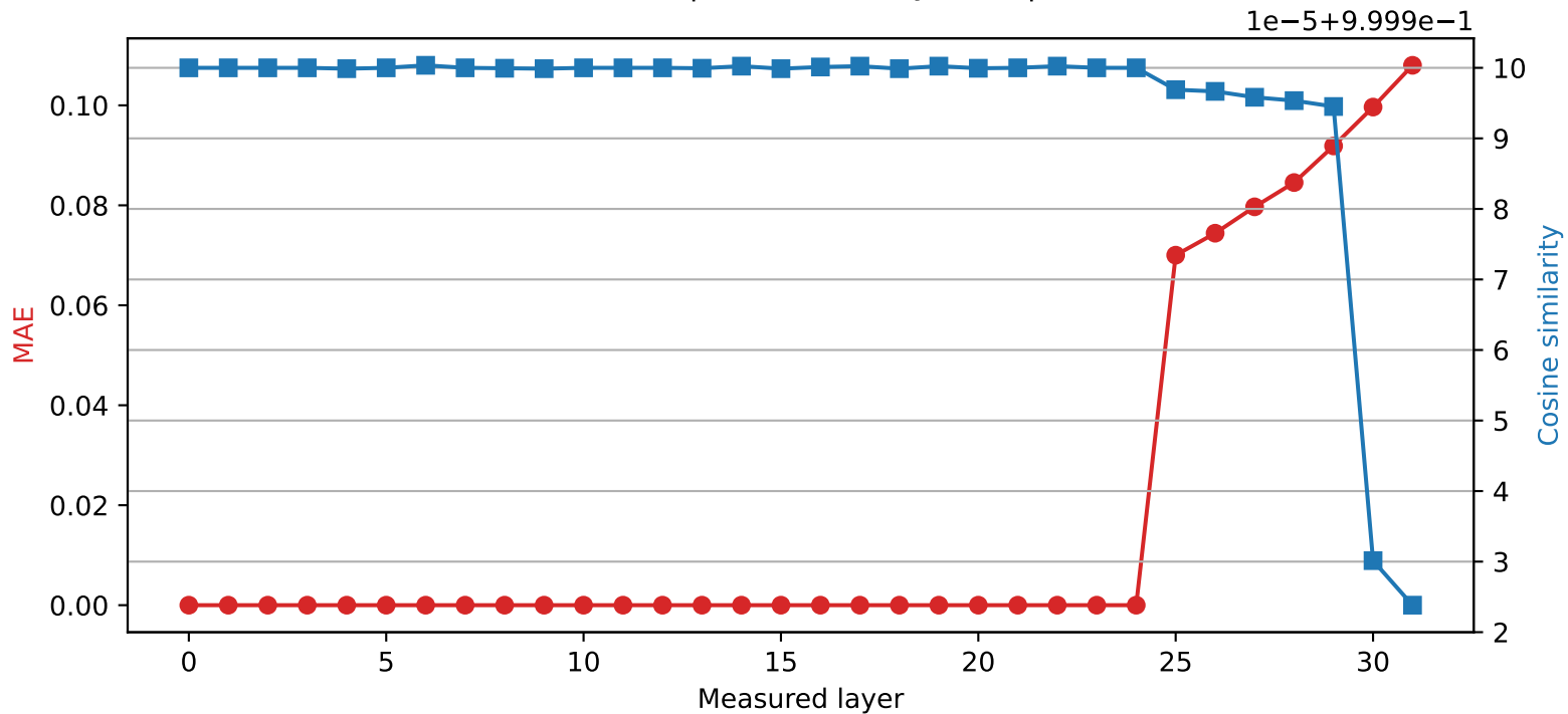
Phi-3-mini-4k-instruct | Quantized layer 24 | float64 → int8
