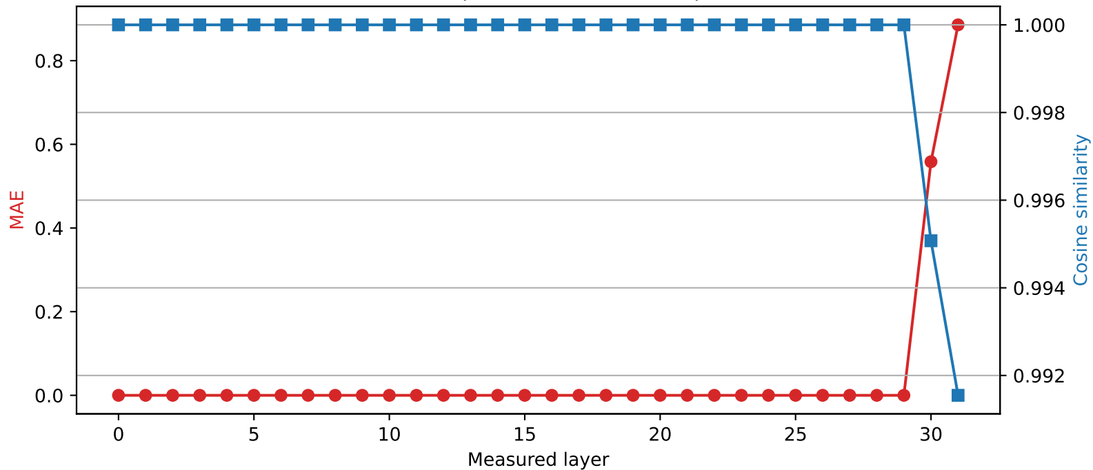
Phi-3-mini-4k-instruct | Quantized layer 29 | float64 \rightarrow int8
