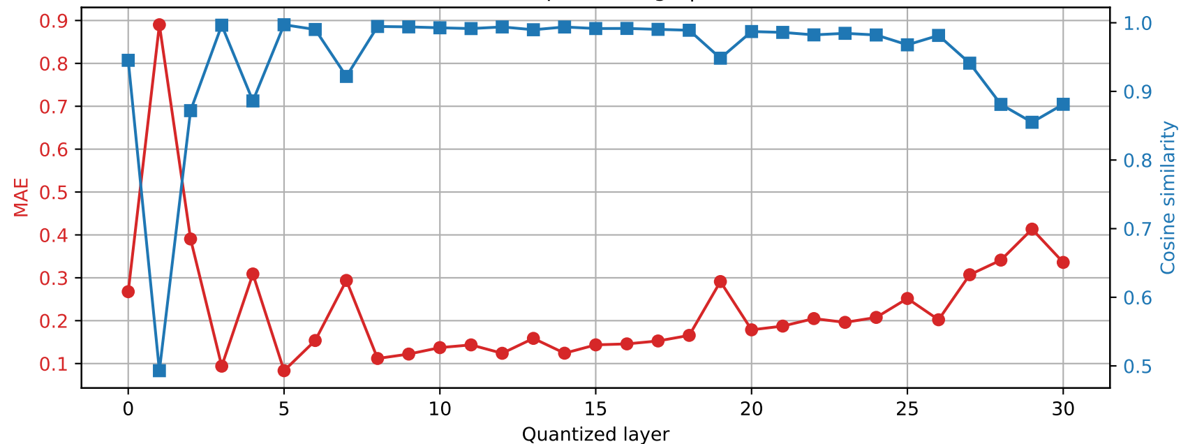
Phi-3-mini-4k-instruct | Prompt 0 Final RMSNorm output damage | float64 \rightarrow int4
