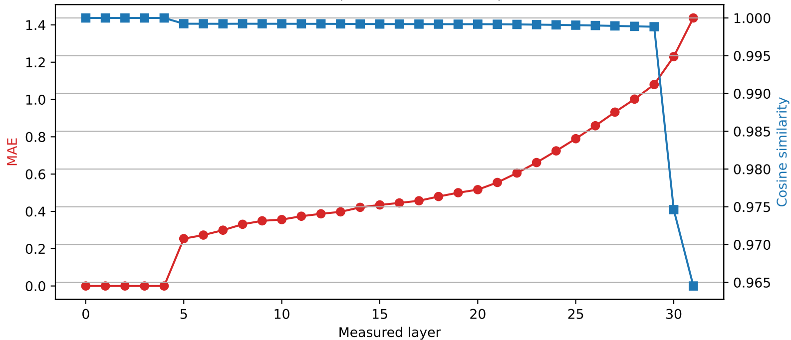
Phi-3-mini-4k-instruct | Quantized layer 4 | float64 \rightarrow int4
