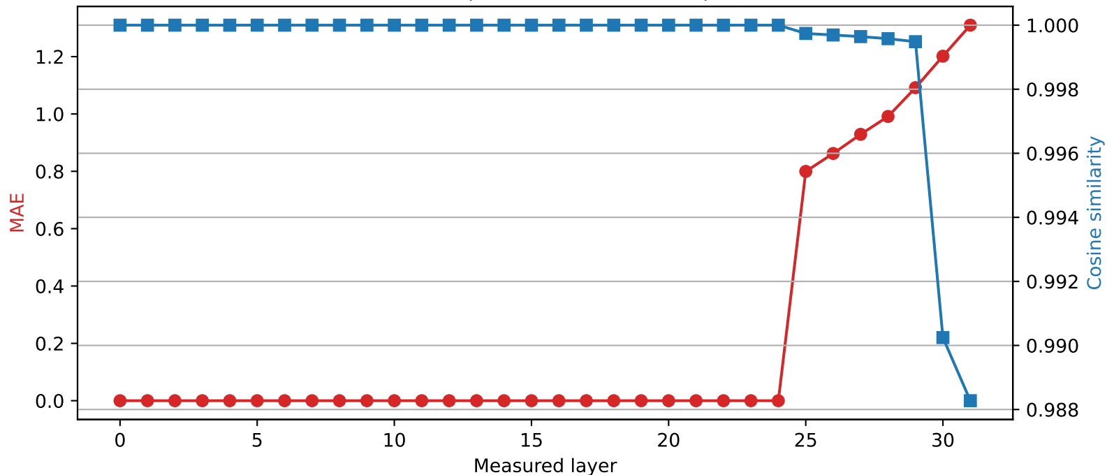
Phi-3-mini-4k-instruct | Quantized layer 24 | float64 \rightarrow int4
