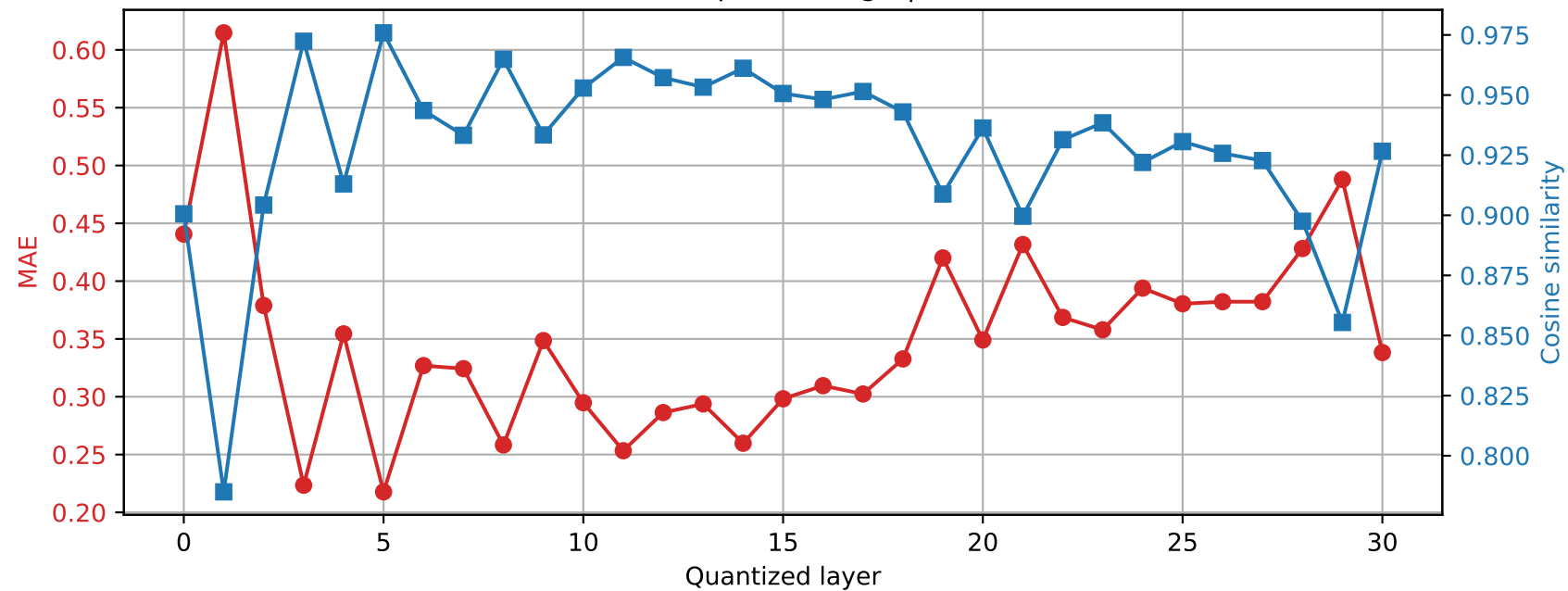
Phi-3-mini-4k-instruct | Prompt 1 Final RMSNorm output damage | float64 \rightarrow int4
