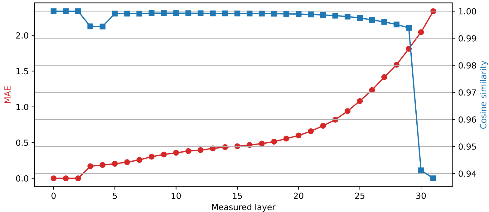
Phi-3-mini-4k-instruct | Quantized layer 2 | float64 \rightarrow int4
