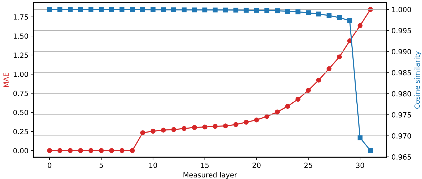
Phi-3-mini-4k-instruct | Quantized layer 8 | float64 \rightarrow int4
