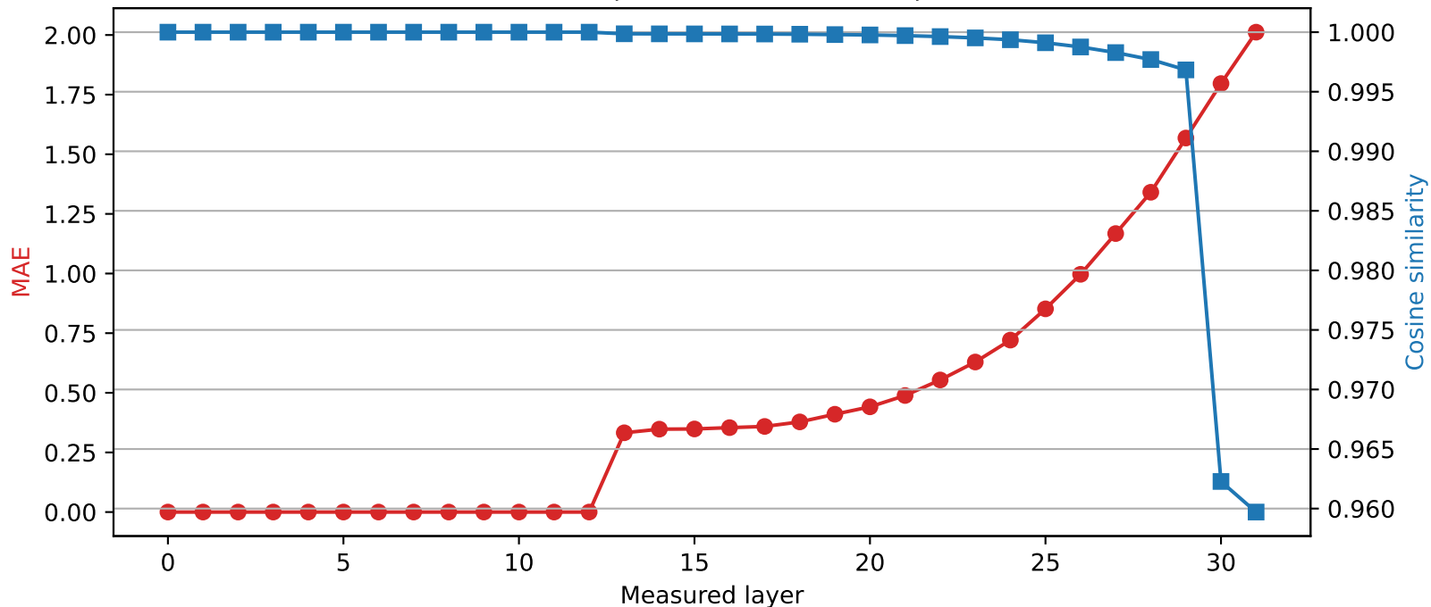
Phi-3-mini-4k-instruct | Quantized layer 12 | float64 \rightarrow int4
